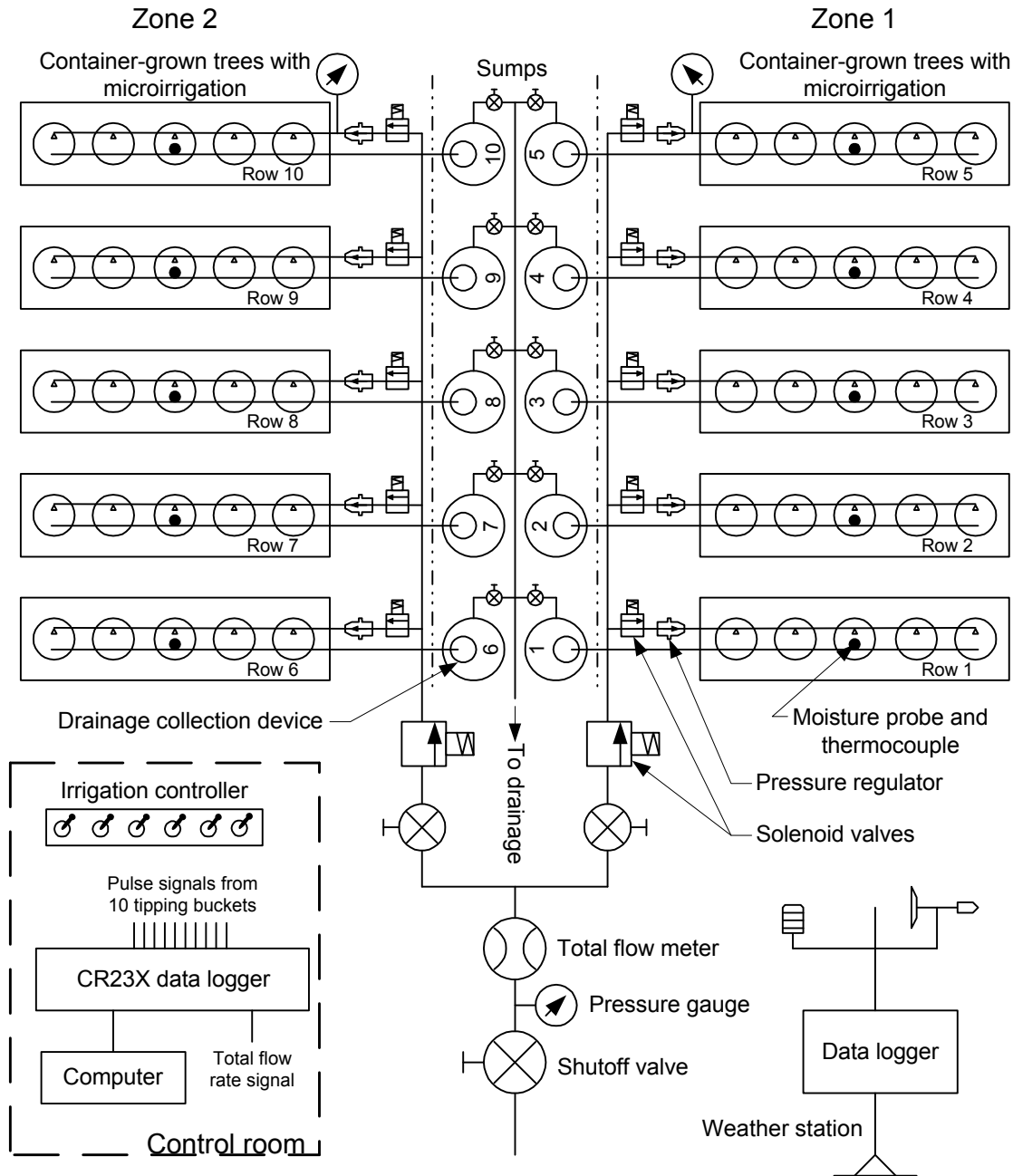
Fig. 1. Schematic diagram of the experimental system for monitoring drainage water quantity and quality, and temperature and water content of container substrate in pot-in-pot nursery production.
